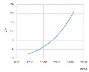
Fuel Consumption
