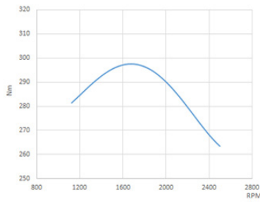
Crankshaft torque
