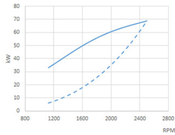
Power (ISO 3046/1)
